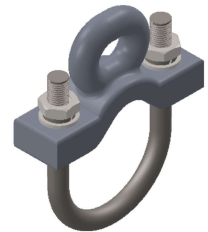
Steady Arm Bracket Assembly
