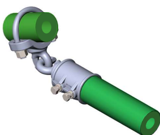
Hook and Eye Type Clamp Assembly
