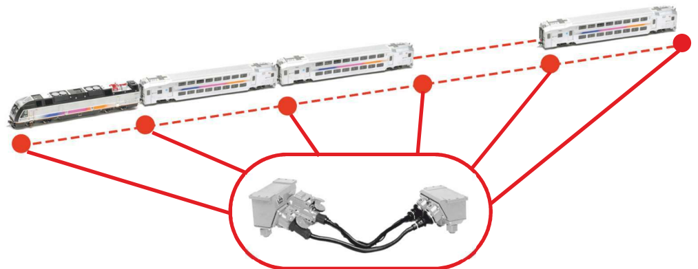
Control Connection Travels through UIC Sockets
