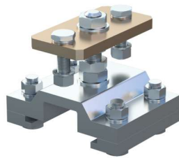
Swivel Head Option-1
