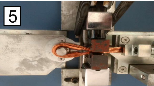
Sleeve crimping
