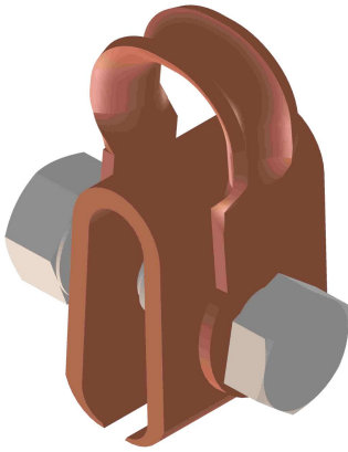
1. Contact Wire Clamp Assembly
