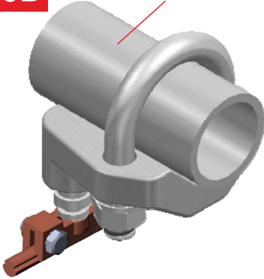
Contact Wire Holder Clamp D-55 Assembly
