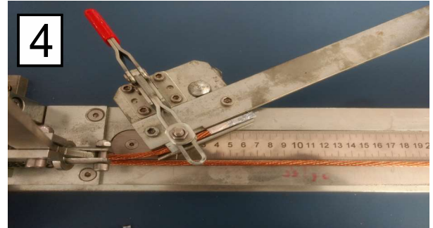
Dropper Straightening
