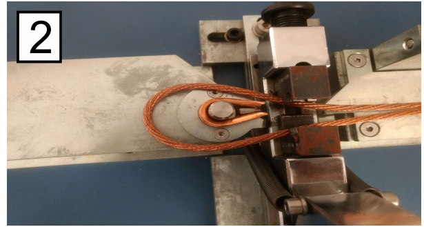
Thimble Placement
