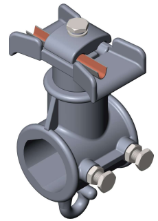
Catenary Wire Support D-55 Assembly with Bimetallic Sleeve
