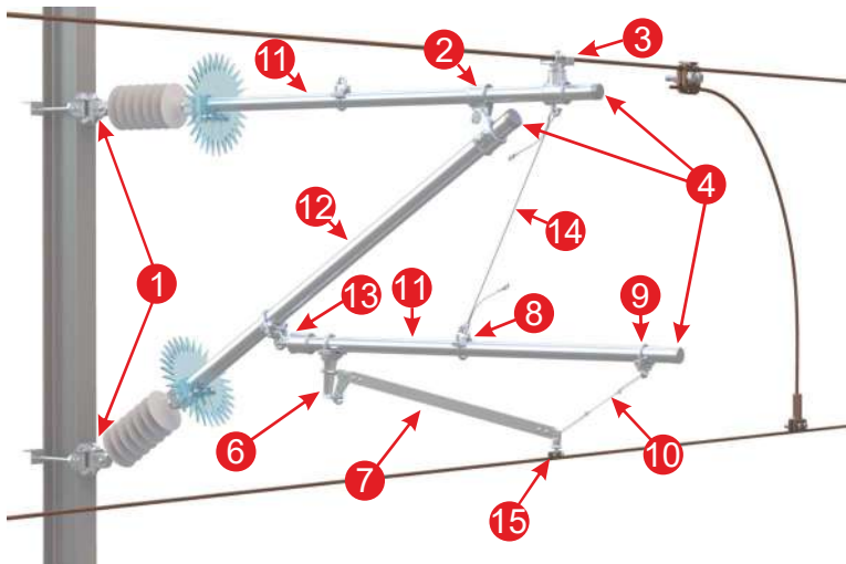
Modular Cantilever System (MCS)
