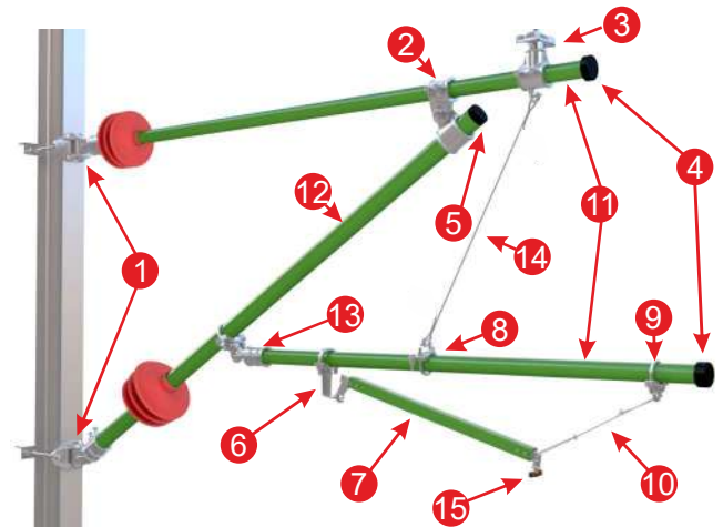
Fully Insulated Modular Cantilever System
