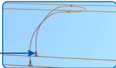
Compression Clamp together with Stay Tube Bracket
