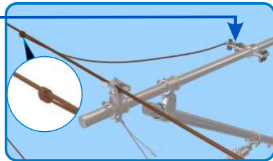
Jumper Stay Tube Clamp
